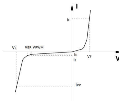
V-I characteristics for a Uni-directional TVS
